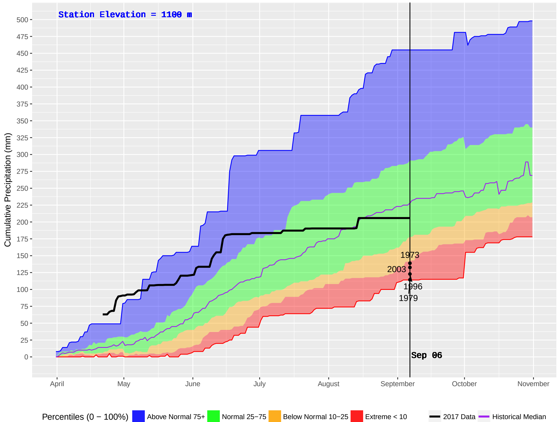
PALLISER (411) : Historical (1973–2016) and Current (2017) Noon Cumulative Precipitation
