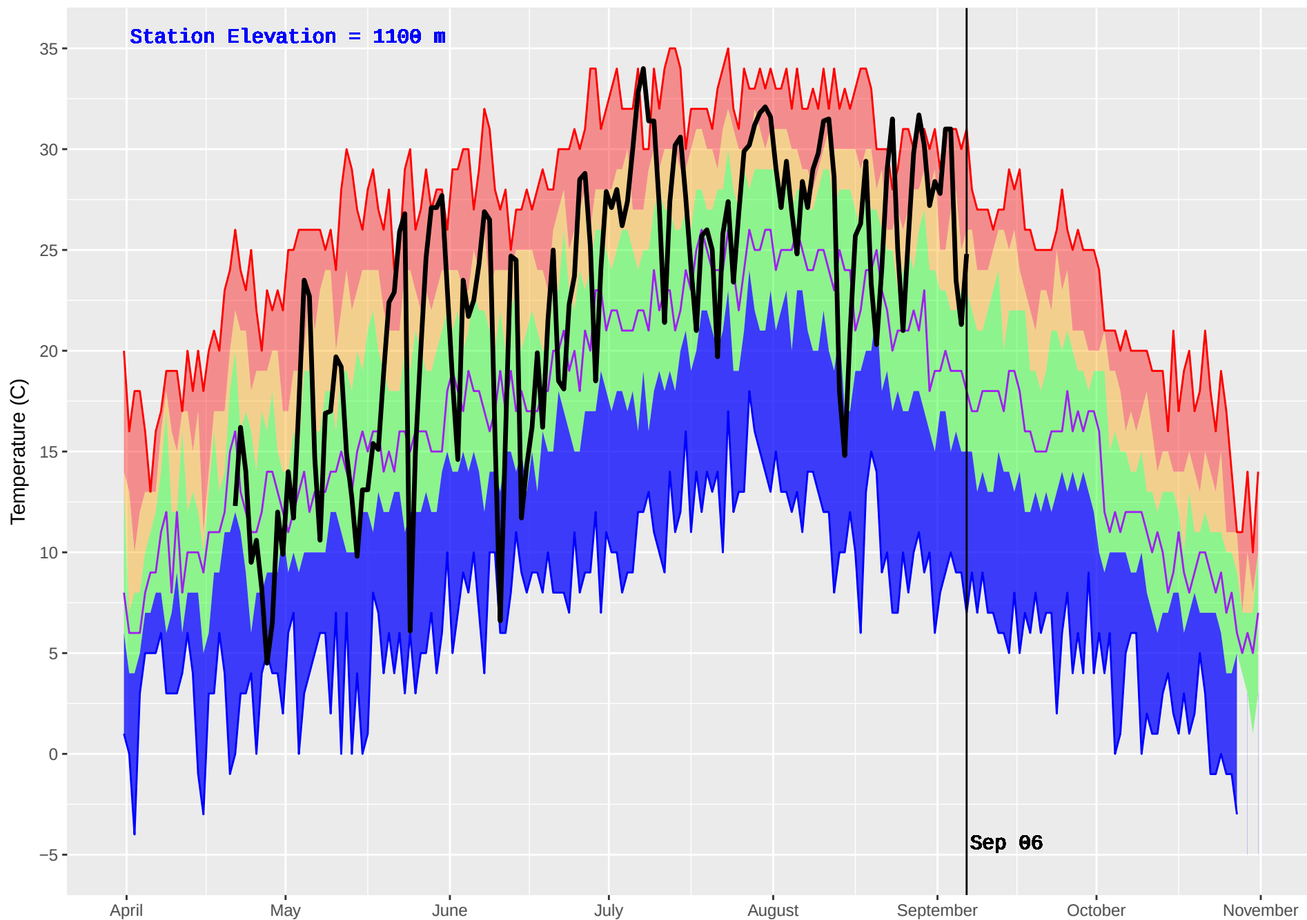
PALLISER (411) : Historical (1973–2016) and Current (2017) Noon Temperature
