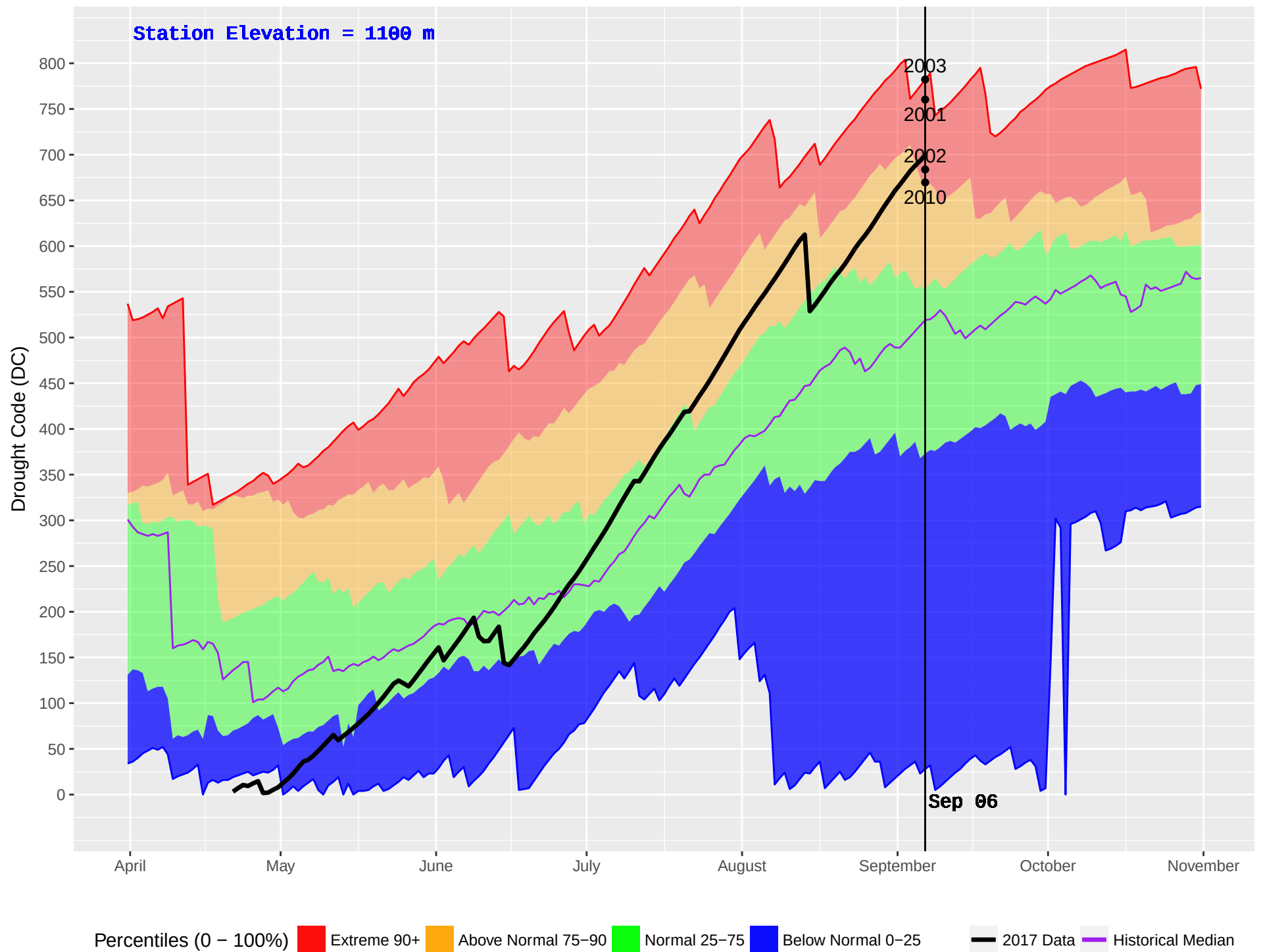
PALLISER (411) : Historical (1973–2016) and Current (2017) Noon Drought Code (DC)
