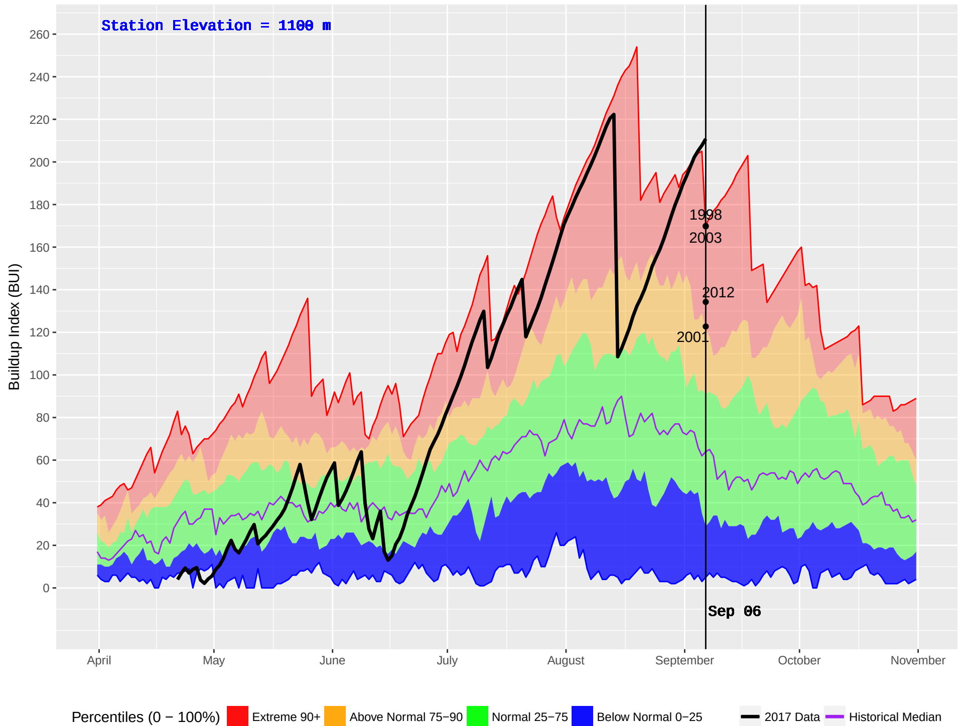
PALLISER (411) : Historical (1973–2016) and Current (2017) Noon Buildup Index (BUI)
